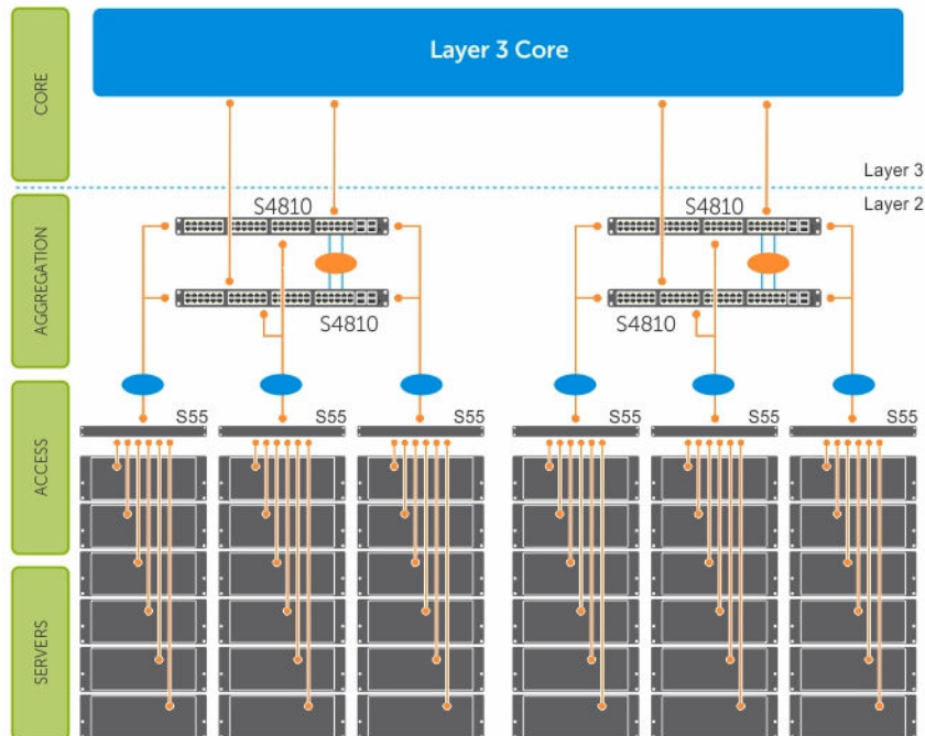
Figure 119. Enhanced VLT
